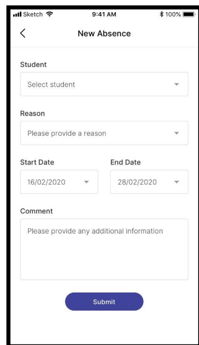
Figure4. View of the New Absence screen
